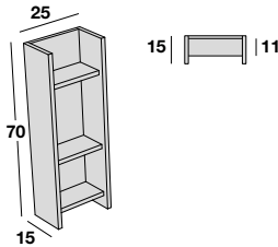
Offener Hochschrank, 3 feste Regale Open column, 3 fixed shelves
