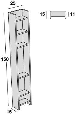
Offener Hochschrank, 6 feste Regale Open column, 6 fixed shelves
